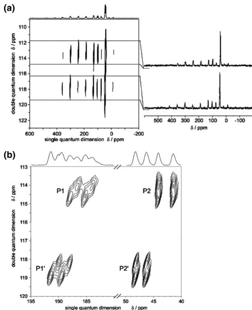
Figure 5. (a) ^{31}\text{P} CP MAS 2D single-quantum double-quantum correlation NMR spectrum of 4f (MAS frequency 4.6 kHz, resonance frequency 81.0 MHz, \text{C9}_1^4 with a Postelement 26 ) showing the resolution of the overlapping spinning sideband patterns of both crystallographically independent molecules. The principal axes values for the P-atoms in the diazaphospholene ring were estimated from the sum projections shown on the right-hand side (see Supporting Information). (b) ^{31}\text{P} CP-MAS INADEQUATE NMR spectrum of 4f (MAS frequency 25 kHz, 2.8 ms double-quantum conversion period, 81.0 MHz resonance frequency) resolving the four multiplets from the two different molecules 4f#1 , 4f#2 in the crystal. The doublet patterns in the direct dimension arise from the ^1J_{\text{PP}} coupling and the complicated splittings (approximately 4:4:1) in the indirect dimension from the coupling to two ^{14}\text{N} atoms in the diazaphospholene ring.
