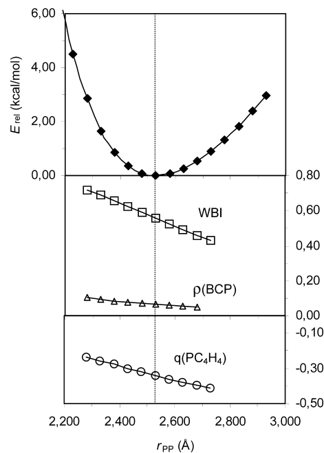
Figure 4. Calculated energies (♦ top), P–P WBI bond index (□), electron densities at the P–P bond critical point (Δ), and sums of NBO charges of the atoms in the phosphole moiety (○) of 7 during a relaxed potential energy scan involving stepwise variation of the P–P distance. All calculations were carried out at the B3LYP/6-31g(d,p)//B3LYP/6-31g(d) level.
