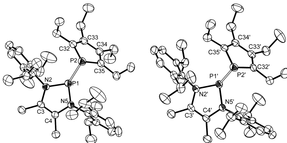
Figure 2. Molecular structure of crystallographically independent molecules 4f#1 (left) and 4f#2 (right) (H-atoms were omitted for clarity; 50% probability ellipsoids). Selected bond lengths (Å) and angles (deg) are given in Table 2 and as Supporting Information.
