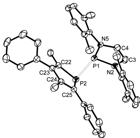
Figure 1. Molecular structure of 4e (H-atoms were omitted for clarity; 50% probability ellipsoids). Selected bond lengths (Å) and angles (deg) are given in Table 2 and as Supporting Information.
